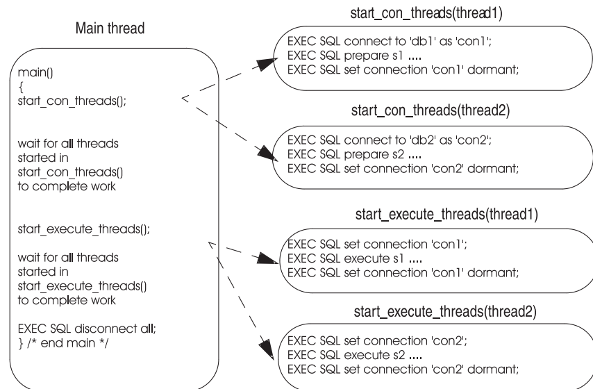
Figure 13-4. Using Prepared SQL Statements Across Threads
