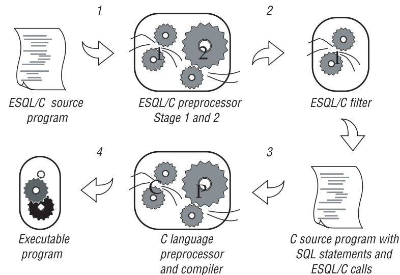
Figure 6-1. Creating an ESQL/C Executable Program from a Non-ASCII Source Program
