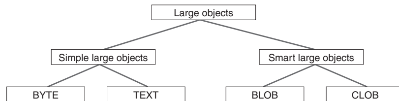
Figure 2-4. Large-Object Data Types
