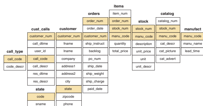
Figure A-1. Joins in the stores_demo Database
