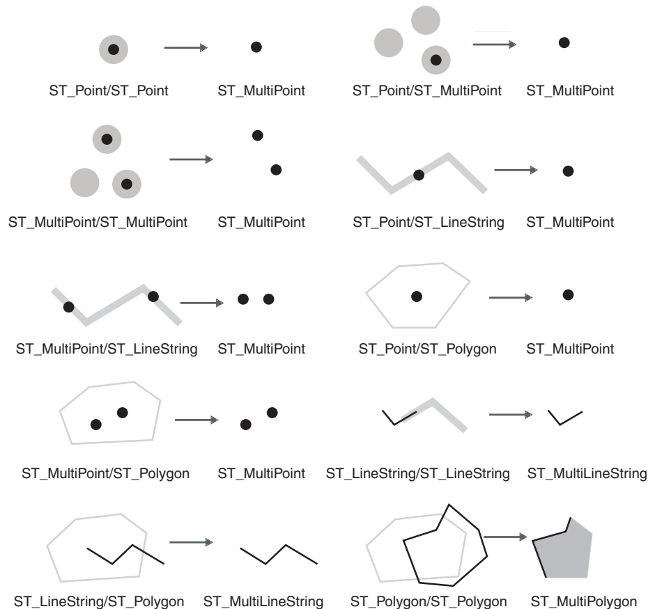
Figure 7-9. Intersection Sets of Geometries
