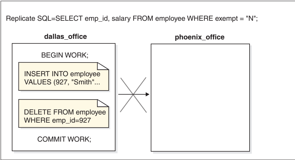
Figure 2-2. Insert Followed by a Delete
