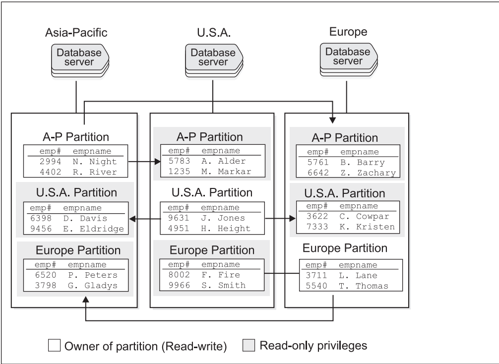
Figure 5-3. Workload Partitioning in a Primary-Target Replication System
