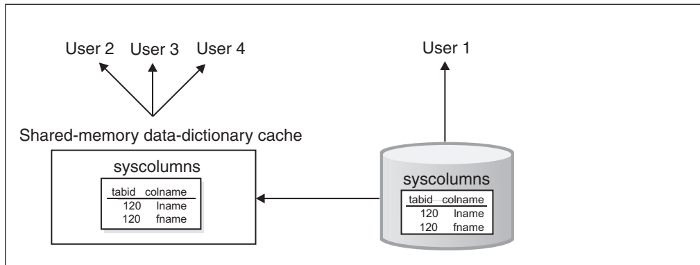
Figure 4-1. Data-dictionary cache
