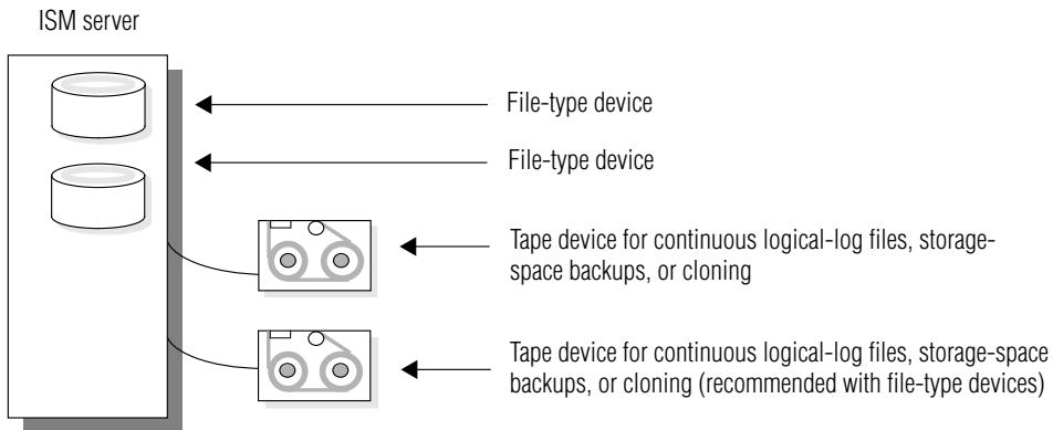
Figure 3-3 ISM Storage-Device Allocation with Two File-Type Devices
