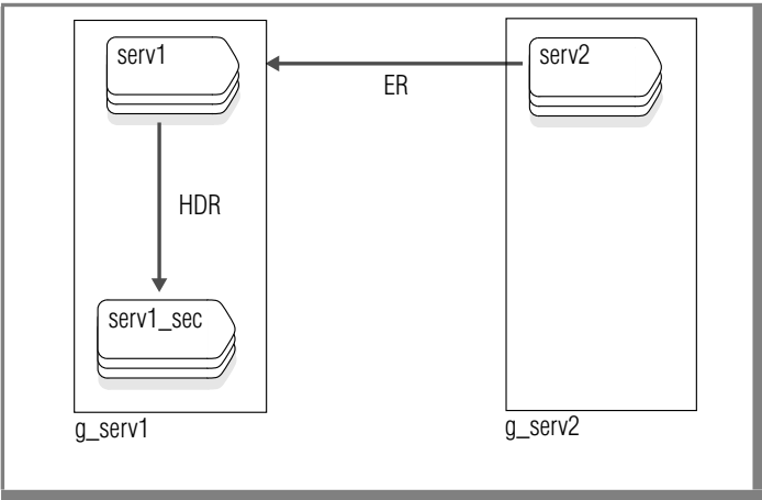
Figure 5-6 Database Server Groups for Enterprise Replication with HDR
