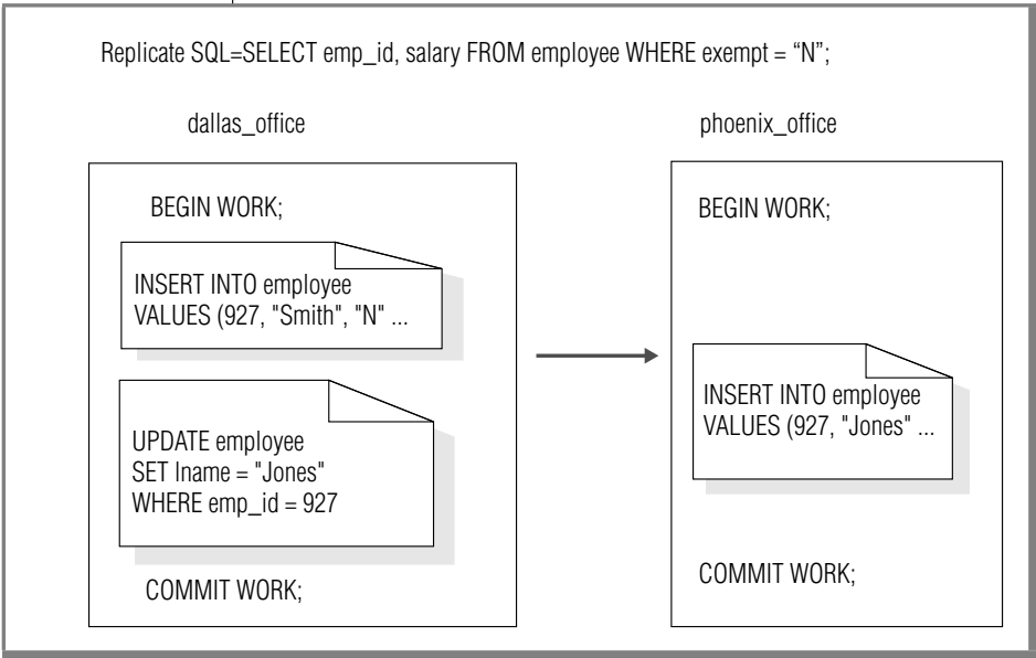
Figure 1-4 Insert Followed by an Update
