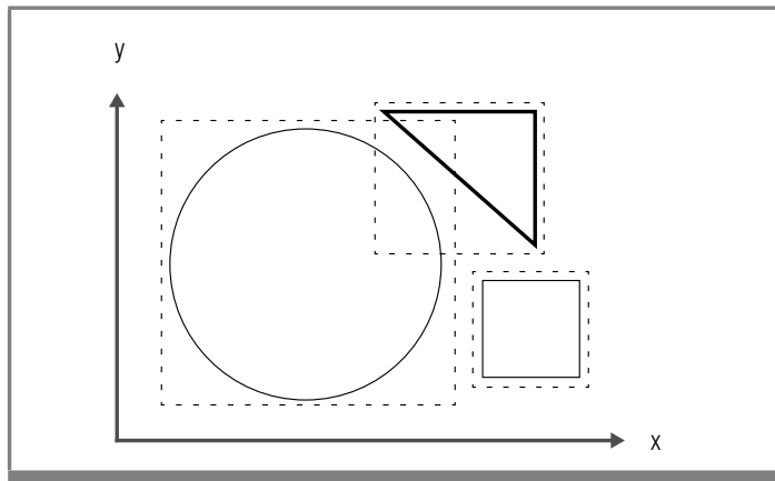
Figure 3-4 Bounding Box Example of the Overlap Function
