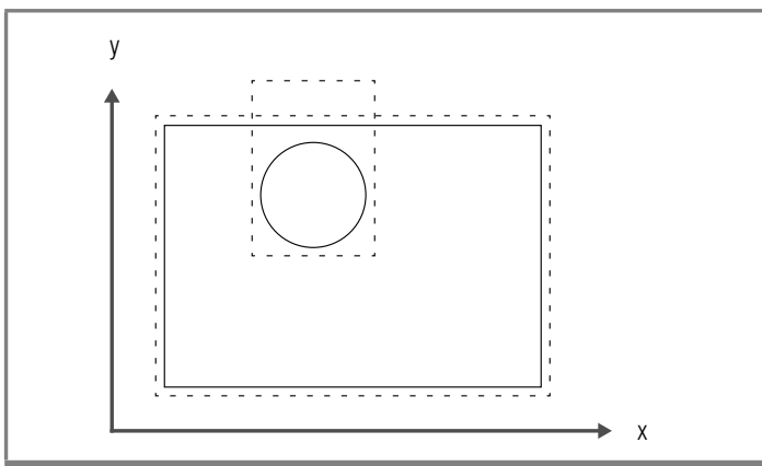
Figure 3-7 Containment and Loose Bounding Boxes
