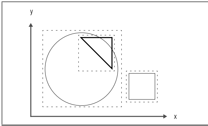
Figure 3-9 Bounding Box Example of the Within Function
