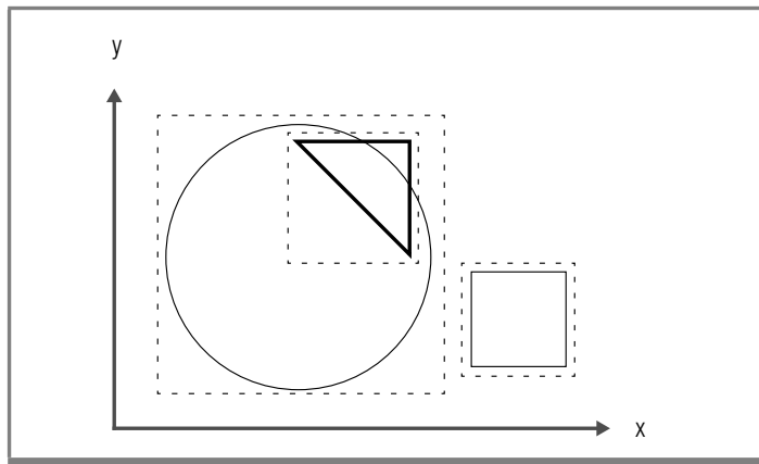
Figure 3-6 Bounding Box Example of the Contains Function
