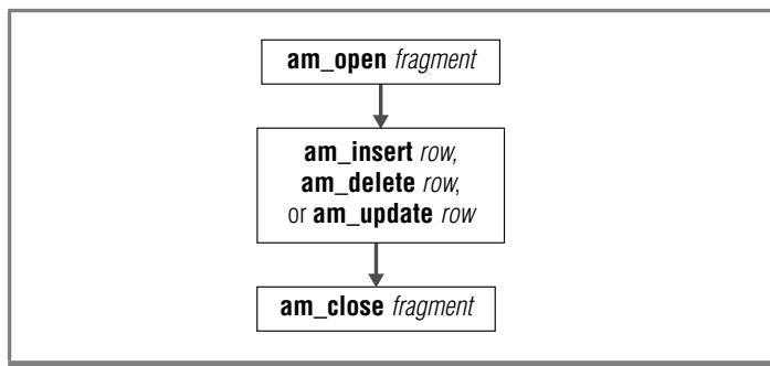
Figure 4-10 INSERT, DELETE, or UPDATE by Row Address
