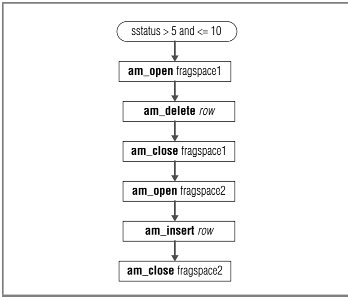
Figure 4-4 Moving Rows Between Fragments
