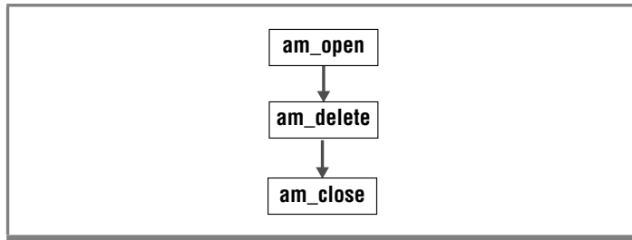
Figure 4-9 Processing a DROP Statement on a Table with a VII Index
