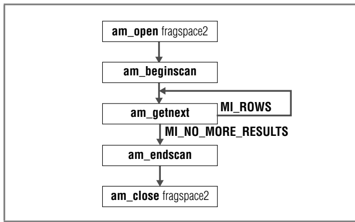
Figure 4-5 Getting All the Rows in Fragment 2
