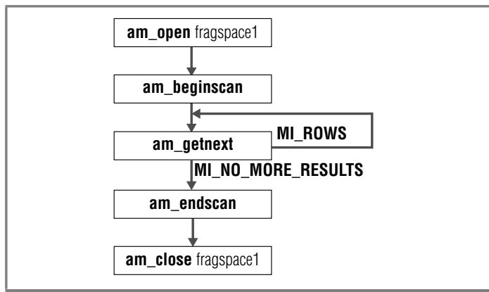
Figure 4-3 Getting All the Rows in Fragment 1
